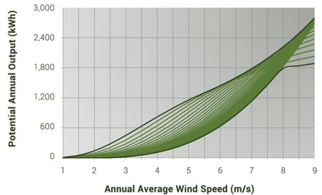
VisionAIR 3 Annual Power Output
