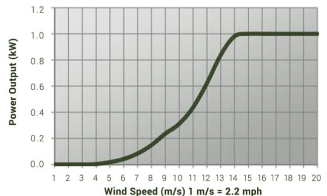
VisionAIR 3 Power Curve
